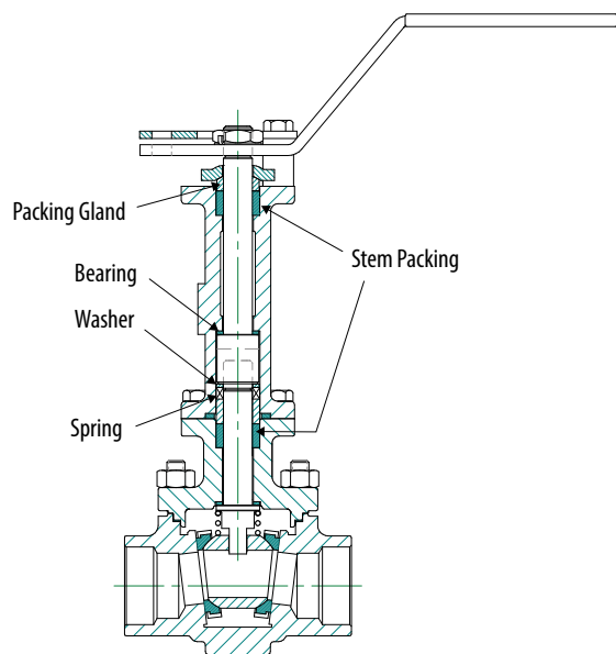
DOUBLE PACKED BONNET (Add "-90" Suffix)
