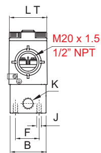
TERMINAL BOX/ Ex d TYPE 16, 19, 37, 39, 58, 58LT
